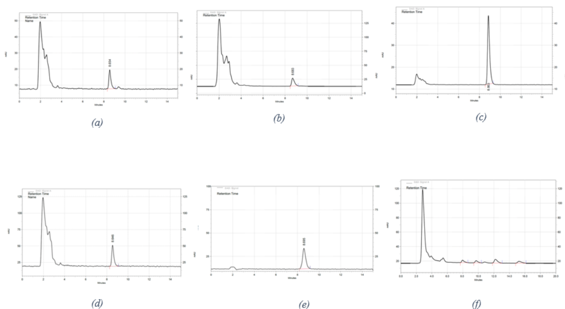
Fig. 2. HPLC Chromatograms of (a) Ergosterol std. (RT=8.654), (b) cordycepin std. (RT=8.683), (c) vitamin d2 std. (RT=8.863), (d) cordycepin sample (RT=8.646), (e) Ergosterol sample (RT=8.695), (f) Vitamin D2 sample
